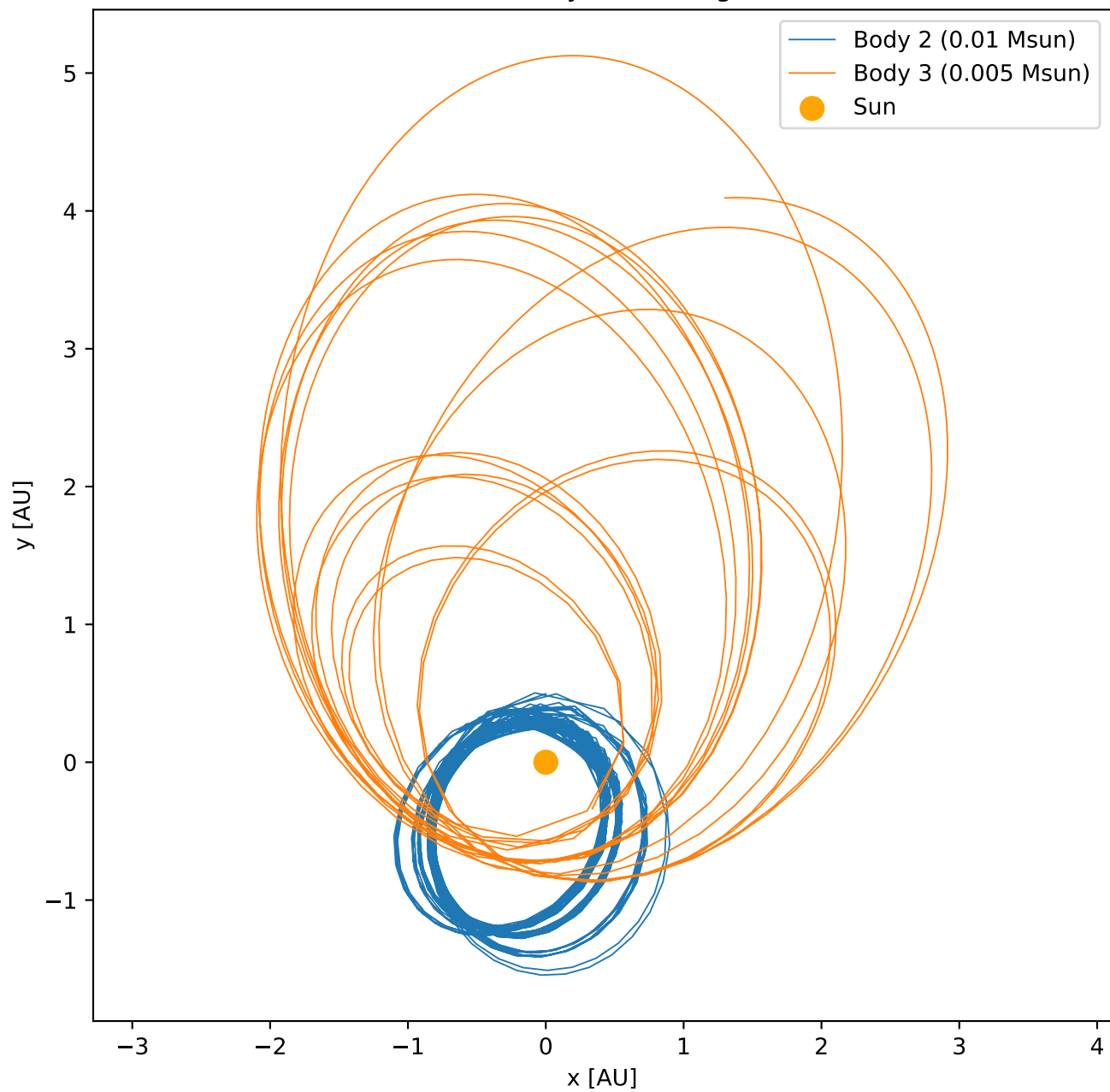
Chaotic Multi-Body Scattering (50 Years)
